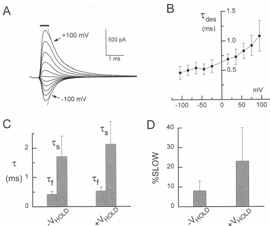
FIGURE 3 Deactivation rates are voltage dependent. (A) Applications (500- \mu s) of 10 mM glutamate to a single patch. Holding potentials were from -100 to +100 mV in 20-mV increments. Same patch as in Fig. 1. The traces at the extreme potentials are shown with single ( -100 mV) and double-exponential ( +100 mV) fits superimposed on the deactivating current. For the fit to the +100 -mV trace, \tau_1 = 0.54 ms, \tau_2 = 2.0 ms, and %SLOW = 13%, whereas the fit for -100 mV was a single exponential of \tau = 0.40 ms. Black bar shows duration of application. (B) Single-exponential time constant of deactivation ( \tau_{off} ) as a function of holding potential. Data from nine patches, in 14-mV bins. Measurements were pooled from applications of 10, 1, and 0.3 mM glutamate (see text). (C) Fast and slow time constants of decay plotted for patches held at -60 to -80 mV ( -V_{HOLD} ) or +60 to +80 mV ( +V_{HOLD} ). Data from six to eight patches. (D) %SLOW (defined in text) for the data set shown in (C).
