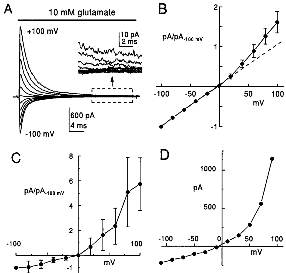
FIGURE 1 Currents activated by 10 mM glutamate at different holding potentials. (A) Glutamate was rapidly applied to an outside-out patch. Bars indicate the duration of drug application. Holding potentials were -100 to +100 mV in 20 -mV increments. The region enclosed by the dashed line (---) is shown enlarged in the inset to illustrate the marked rectification of the steady-state currents. (B) I-V relation for peak current response to 10 mM glutamate. Peak currents evoked by 10 mM glutamate in five patches were normalized to the current at the potential nearest -100 mV and plotted against holding potential. Data were binned into 7 -mV bins. To emphasize the extent of rectification, the dashed line (---) represents a linear regression over the points at the five most negative potentials. The estimated reversal potential from this fit is -0.43 mV. (C) I-V relation for the steady-state response in five patches after 30 ms of exposure to 10 mM glutamate. Data were binned as in (B) and normalized to the response at -100 mV. (D) Steady-state current obtained from a whole cell in response to voltage jumps ( -100 to +90 mV, leak subtracted) in the presence of 1 mM glutamate, showing that outward rectification persists in intact cells.
