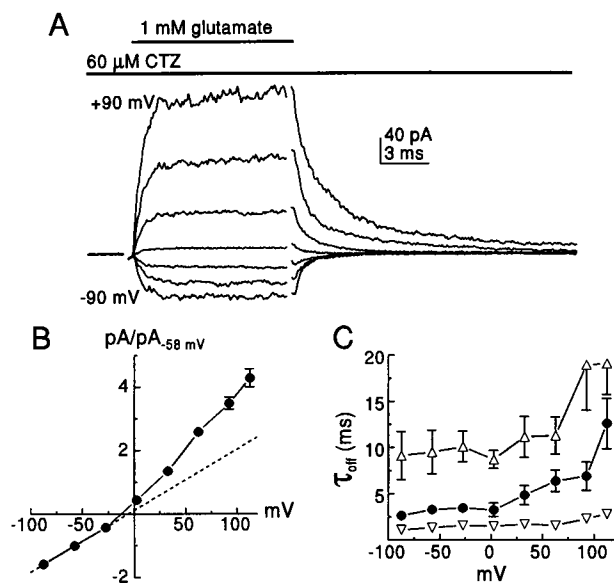
FIGURE 5 Rectification persists in the presence of cyclothiazide. (A) Responses of a patch to 1 mM glutamate in the presence of 60 \mu M cyclothiazide. Holding potentials were -90 mV to +90 mV in 30-mV steps. Each trace is an average of five records. (B) Maximal currents from eight patches were normalized to the current evoked at the holding potential nearest -58 mV (11-mV bins). The dotted line ( \cdots ) is a linear regression over the data at the three most negative potentials, and it has a slope of 0.019 and a y-intercept of 0.11. The reversal potential is therefore estimated at -5.8 mV. (C) Deactivation time constants versus holding potential; data from eight patches as in (B). Bars are standard errors. Filled symbols ( \bullet ) represent values from single-exponential fits. Triangles show the time constants from double-exponential fits, with the inverted ( \nabla ) and upright ( \Delta ) triangles representing the fast and slow components, respectively.
