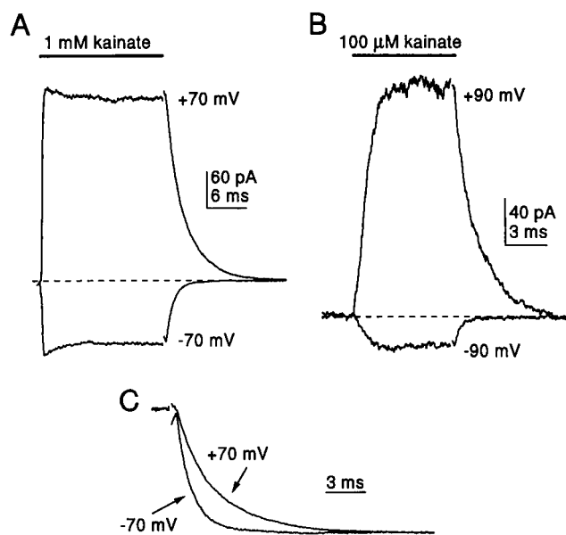
FIGURE 4 Rectification of kainate-evoked currents. (A) Kainate (1 mM) was applied to a patch held at -70 mV and +70 mV. The dashed line (---) indicates 0 current. Mean of 16 records. (B) Kainate (100 \mu M) was applied to a patch, different from the one in (A). Holding potentials were +90 and -90 mV. Mean of five records. (C) Current offsets from (A) are normalized to the maximal current in each trace in order to illustrate the slower deactivation at positive potentials. The time constants (in milliseconds) from a double-exponential fit to the deactivating phase and the relative contributions of the two components at -70 mV were \tau_{fast, off} = 0.87 , \tau_{slow, off} = 1.81 , %SLOW = 30%; at +70 mV, \tau_{fast, off} = 1.23 , \tau_{slow, off} = 3.52 , and %SLOW = 68%.
